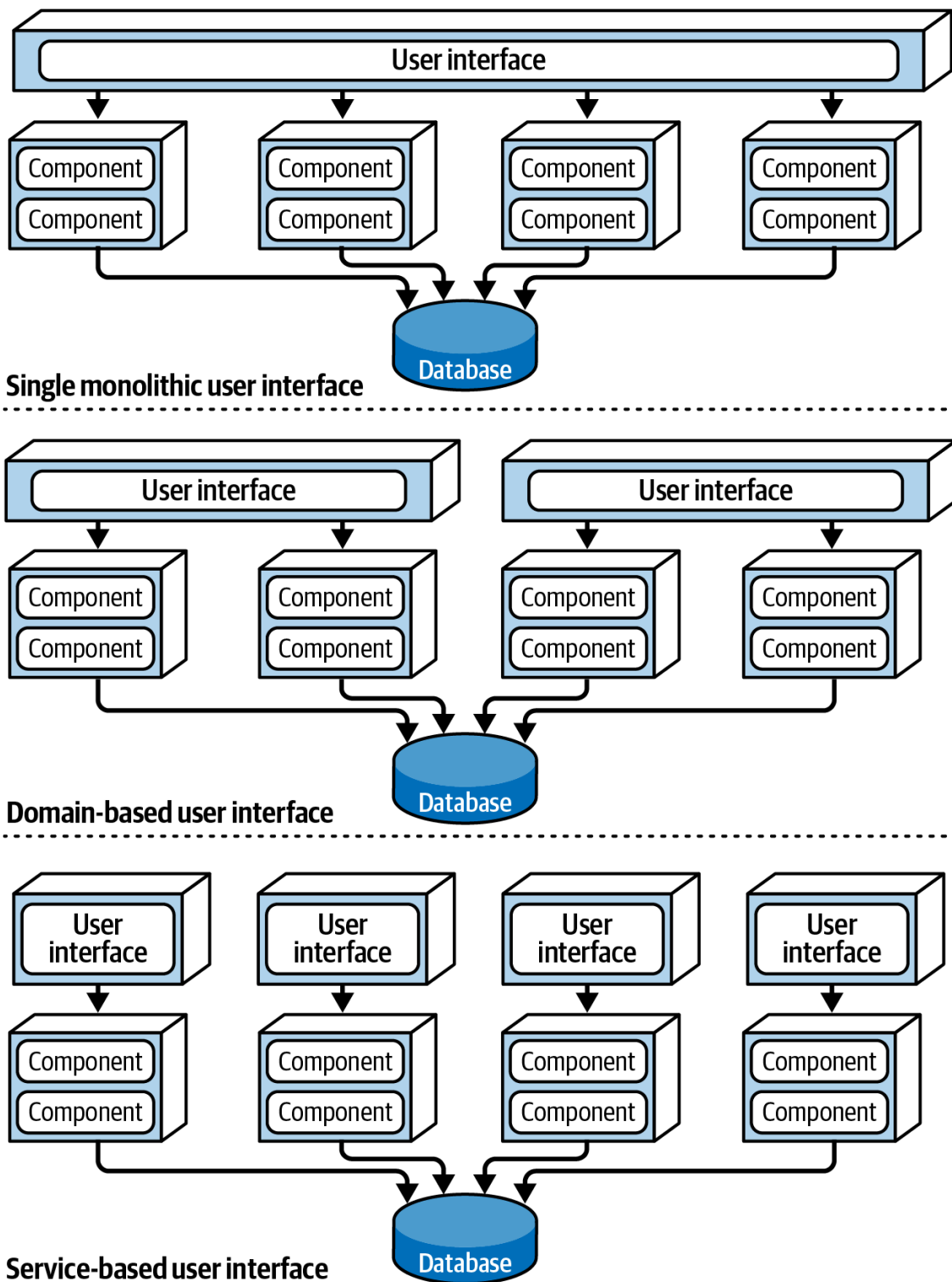
Figure 14-3. Three user-interface variants in a service-based architecture
